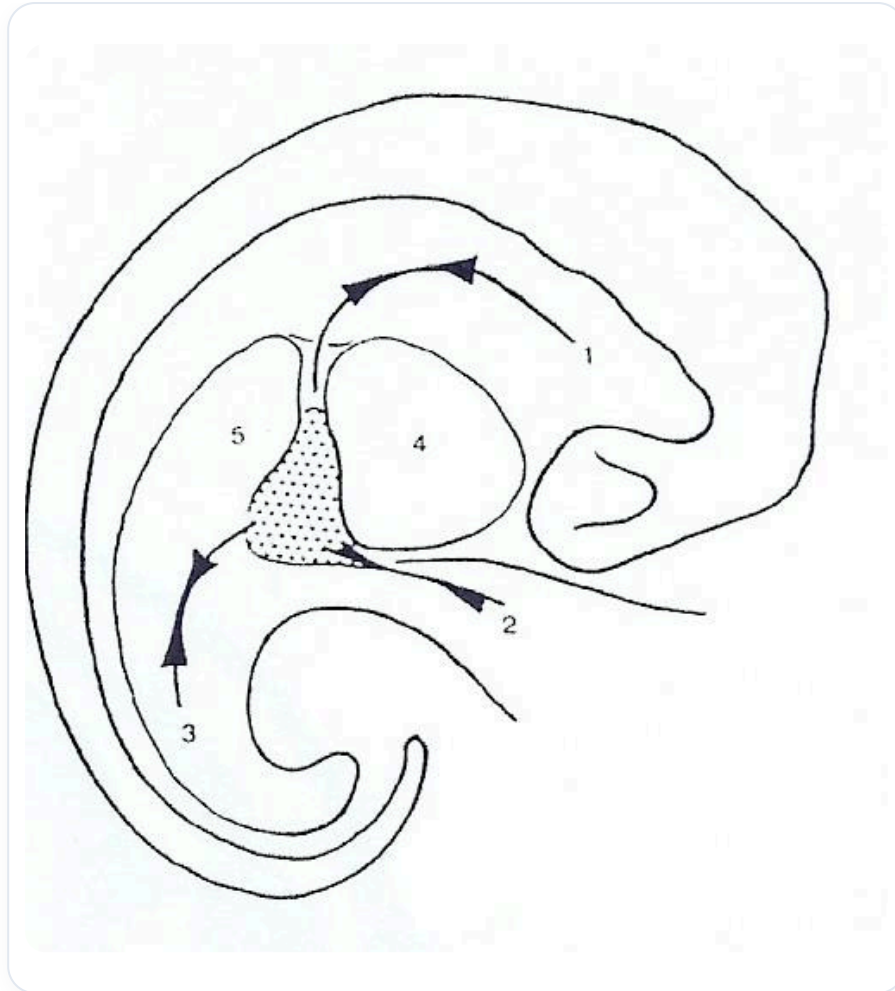
ABB. — Circulation embryo liquide
